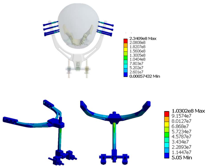
Fig. 4 Stress distribution of external distractor device component of the new hybrid distractor device.
