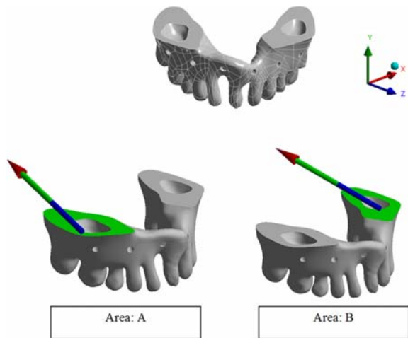
Fig. 7 Reaction force during maxillary distraction osteogenesis.
