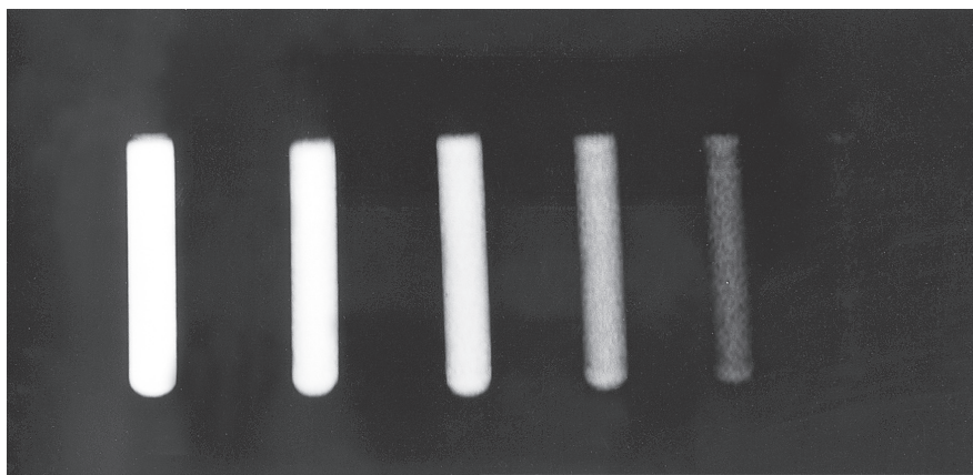
Fig. 2 Roselle flower tea (RFT) phantom was scanned with standard MRCP technique and showed that signal intensity of the tube with 100% RFT concentration appeared equal to the background noise. Other tubes shows increased signal intensity as the concentration reduced
