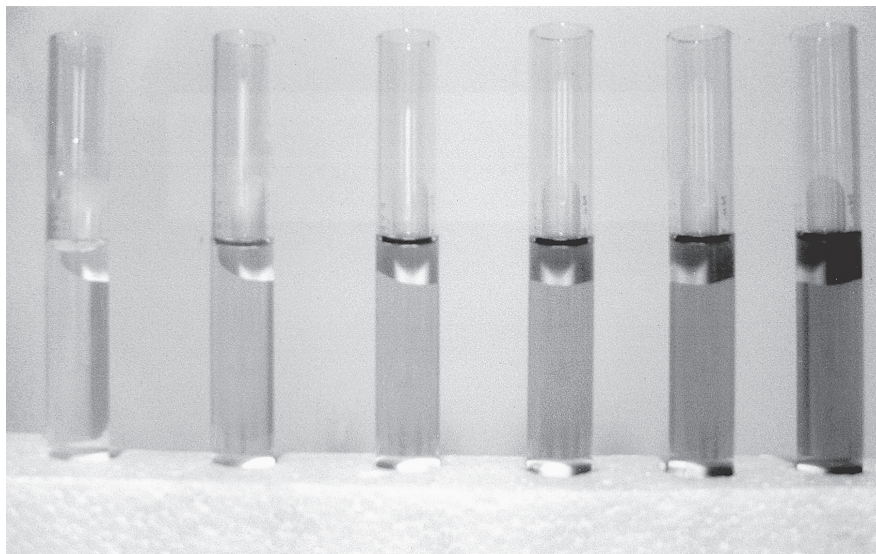
Fig. 1 Roselle flower tea (RFT) phantom. The far right tube is 100% concentration of RFT. The far left tube is distilled water. Other 4 tubes are RFA with diluted concentration of 80%, 60%, 40% and 20% from right to left, respectively
